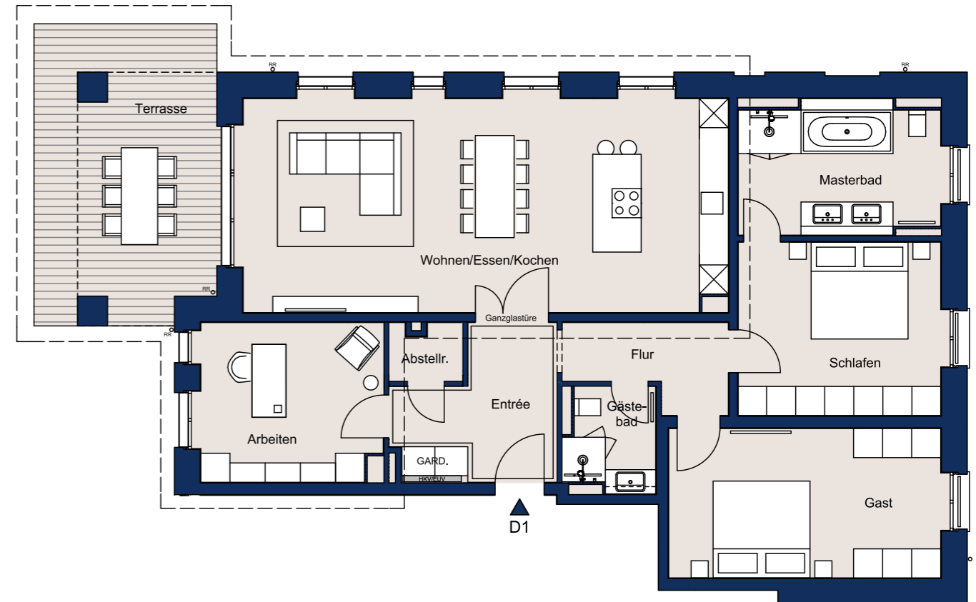
Grundrissalternative
